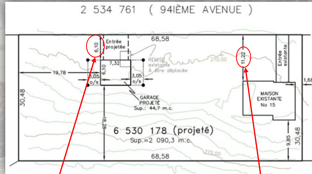
Implantation
