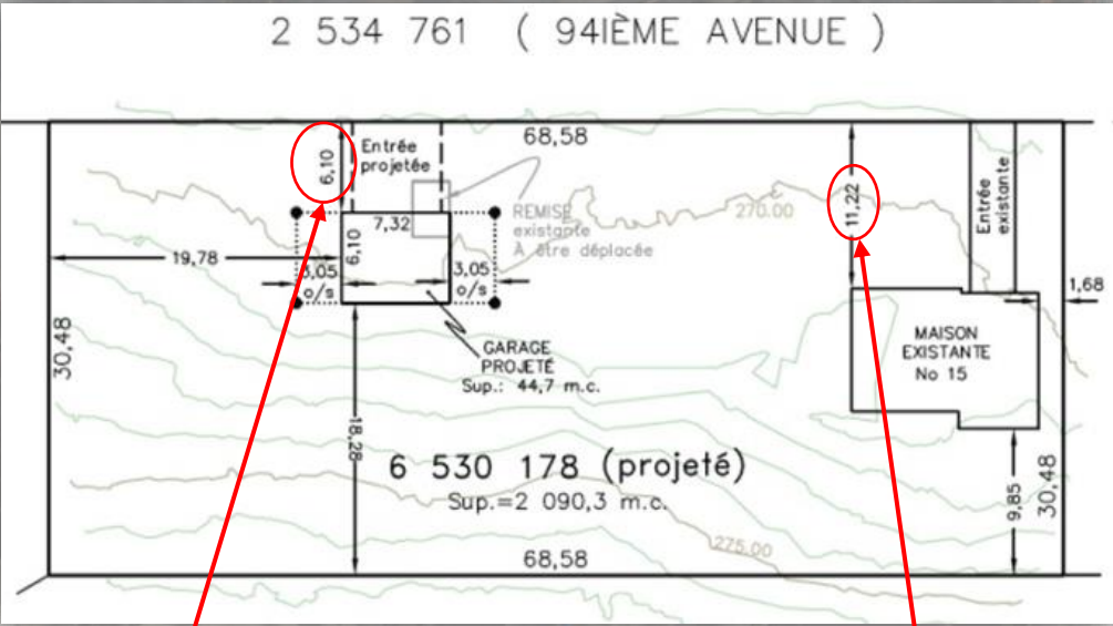
Implantation
